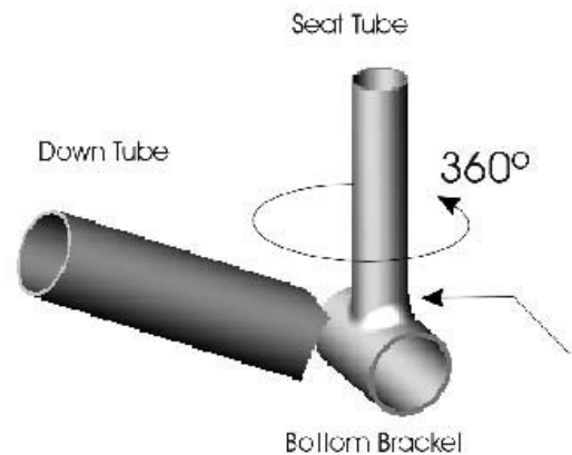
Figure 3: Proper Attachment of Seat Tube to Bottom Bracket
