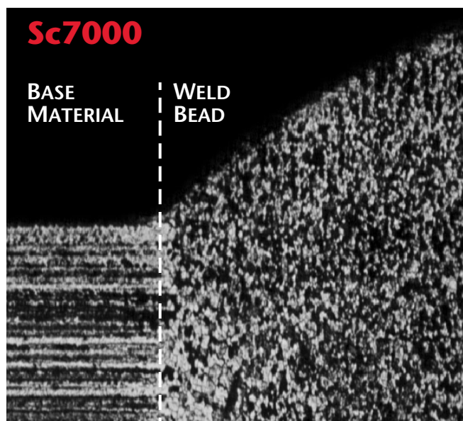
Figure 1: SC7000 Base Material and Scandium Weld Rod
