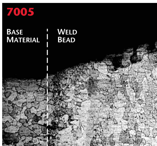
Figure 2: 7005 Base Material and 5356 Filler Rod
