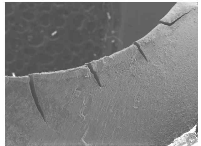
Figure 6: SEM Photograph Showing Mechanical Deformation Caused by Over-Torqued Rivet Nut
